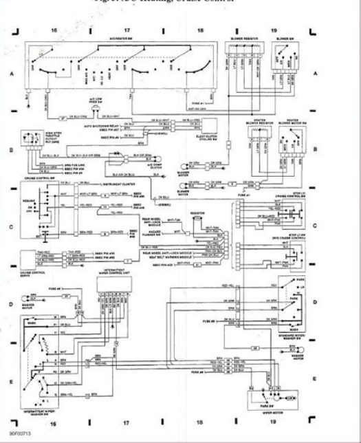
Fig. 5: A/C-Heating, Cruise Control
